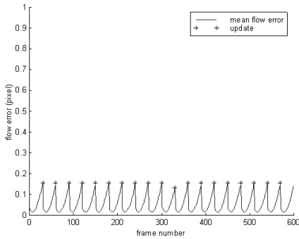
Figure 4: MSE for R_x and R_y
