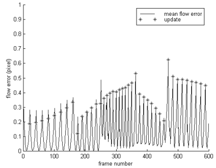
Figure 6: MSE for full motion
